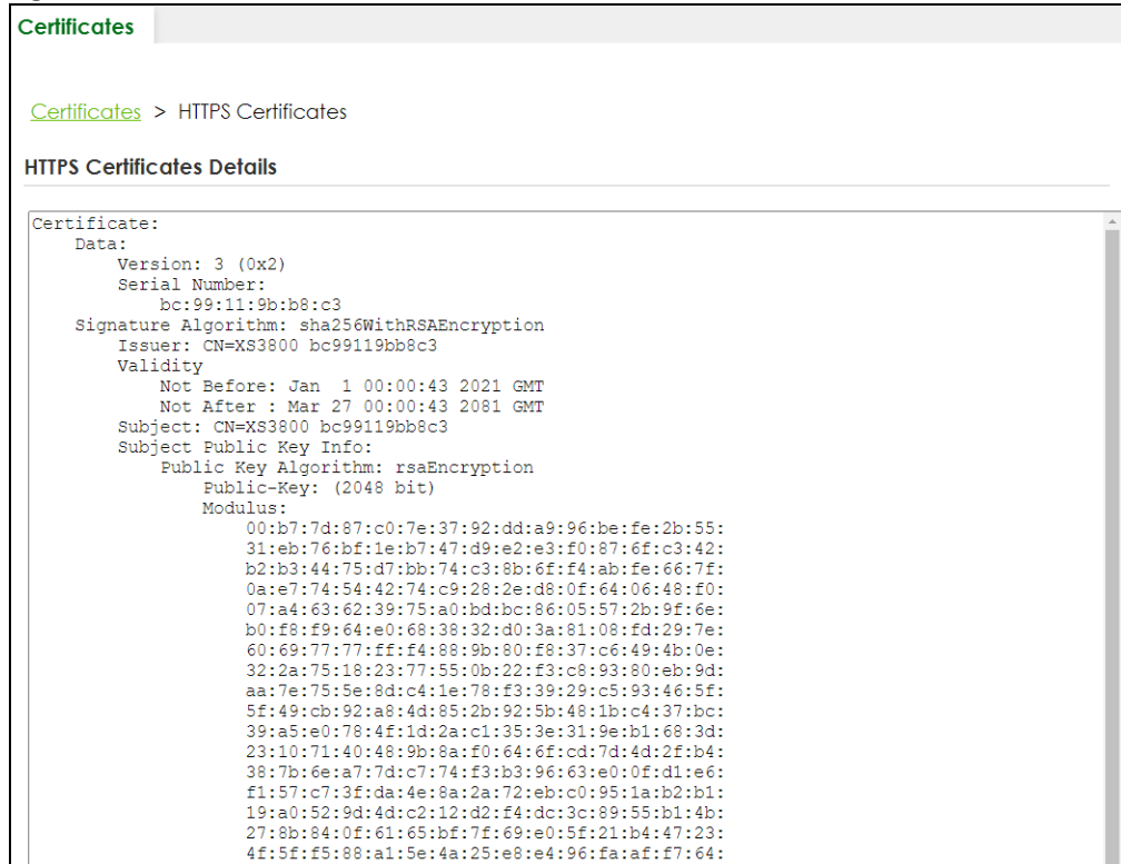
Figure 393 MAINTENANCE &gt; Certificates &gt; HTTPS
