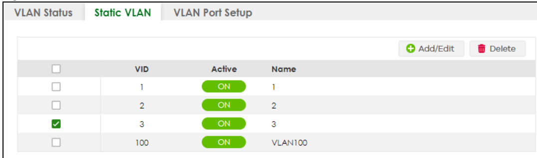
Figure 450 SWITCHING > VLAN > Static VLAN
