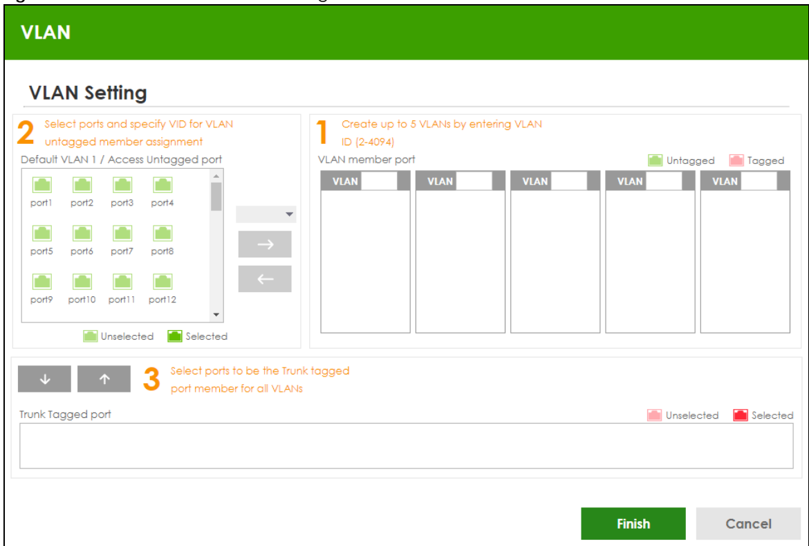
Figure 62 Wizard > VLAN > VLAN Setting
