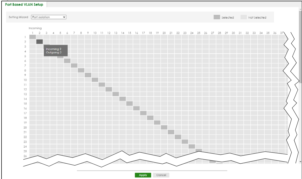
Figure 288 SWITCHING &gt; VLAN: Port Based VLAN Setup (Port Isolation)
