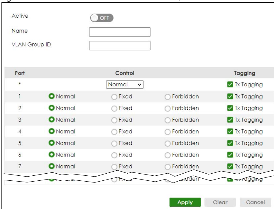
Figure 451 SWITCHING > VLAN > Static VLAN > Add/Edit
