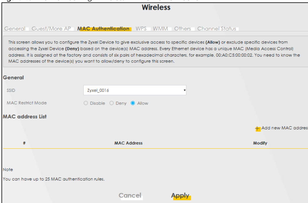
Figure 48 Network Setting> Wireless > MAC Authentication
