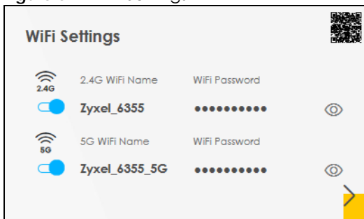
Figure 51 WiFi Settings
