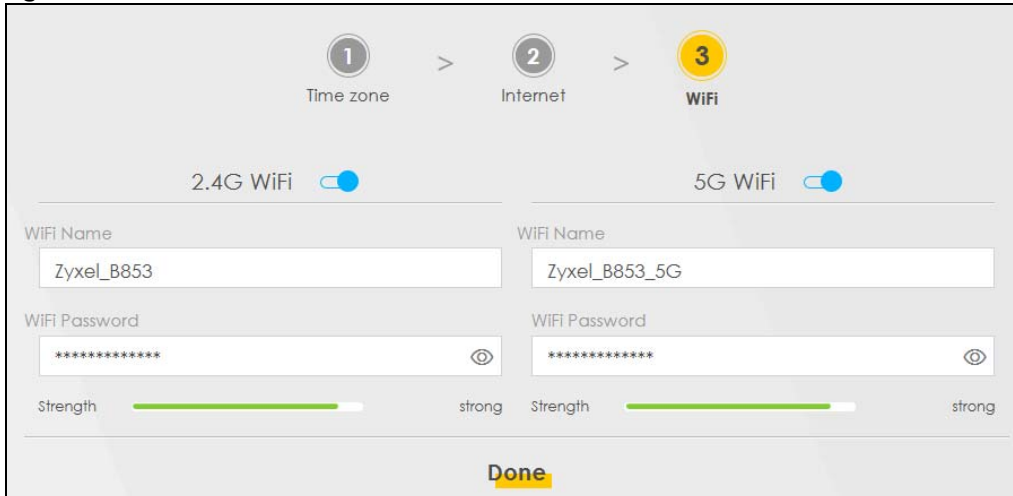
Figure 41 Wizard - Wireless
