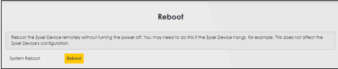
Figure 194 Maintenance > Reboot
