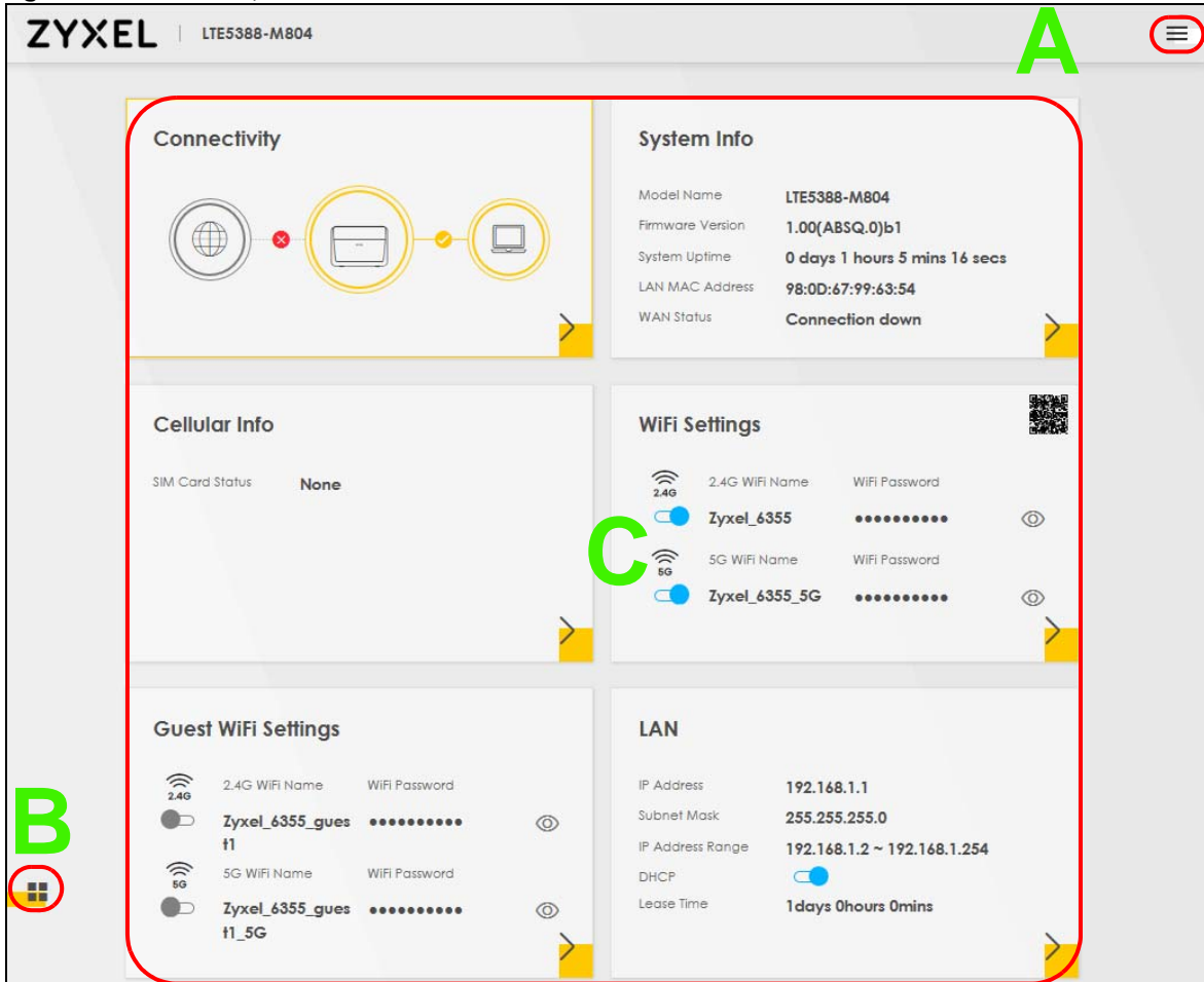
Figure 31 Screen Layout
