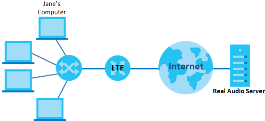
Figure 124 Trigger Port Forwarding Process: Example
