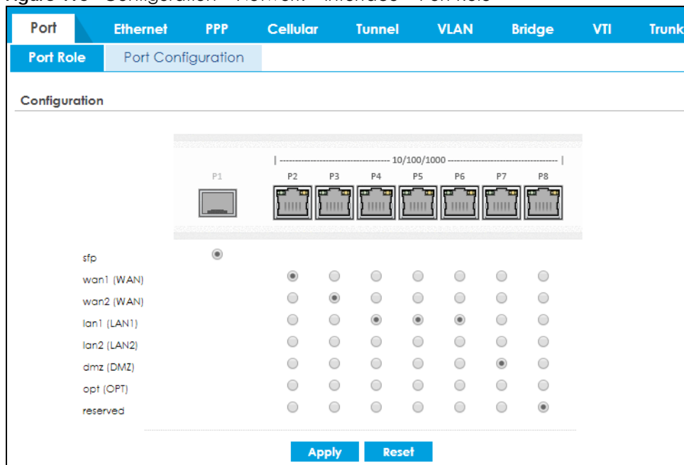
Figure 193 Configuration > Network > Interface > Port Role
