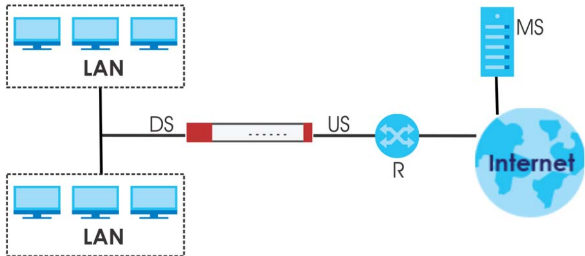
Figure 196 IGMP Proxy
