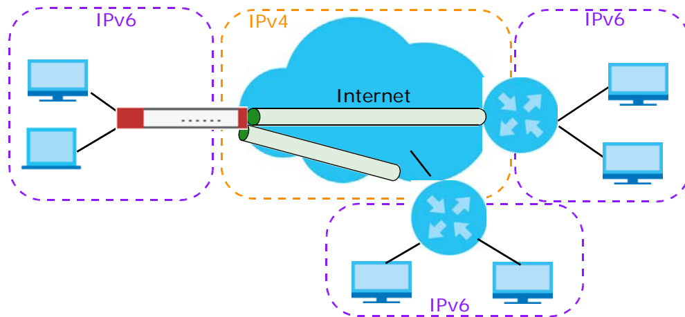
Figure 214 6to4 Tunnel
