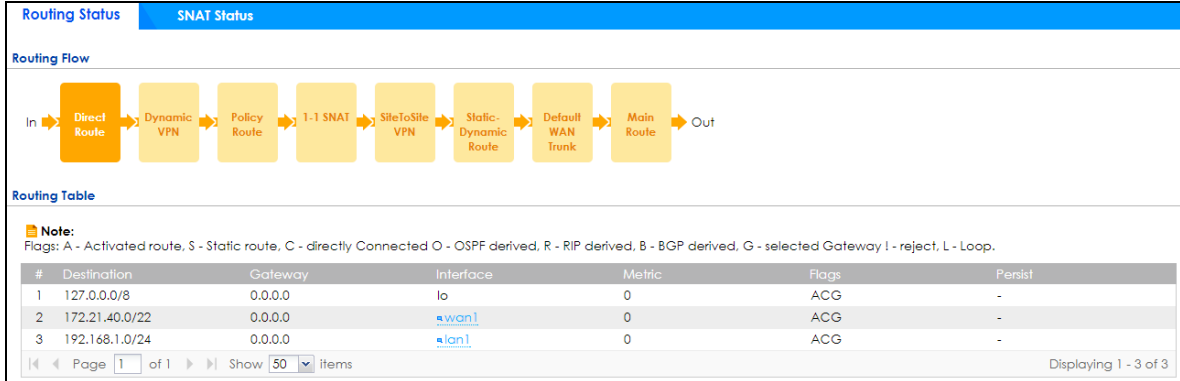
Figure 607 Maintenance > Packet Flow Explore > Routing Status (Dynamic VPN)
