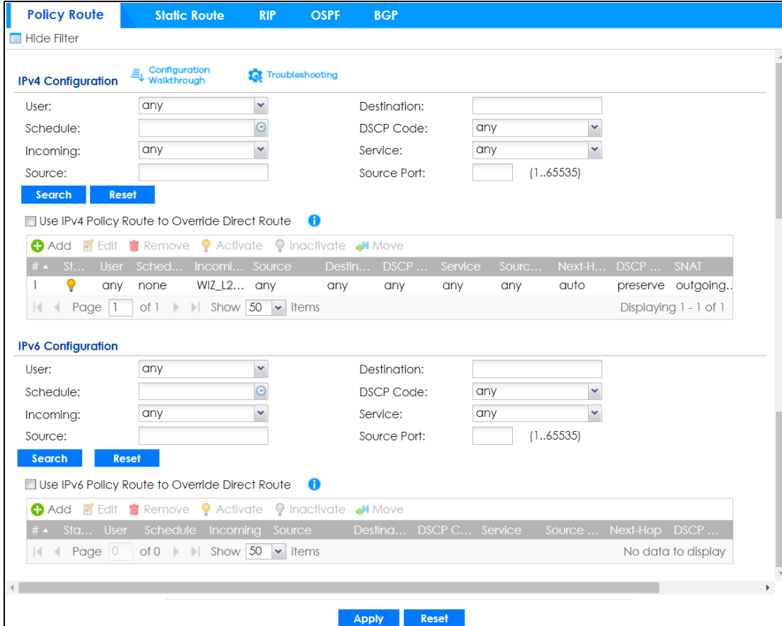
Figure 234 Configuration > Network > Routing > Policy Route
