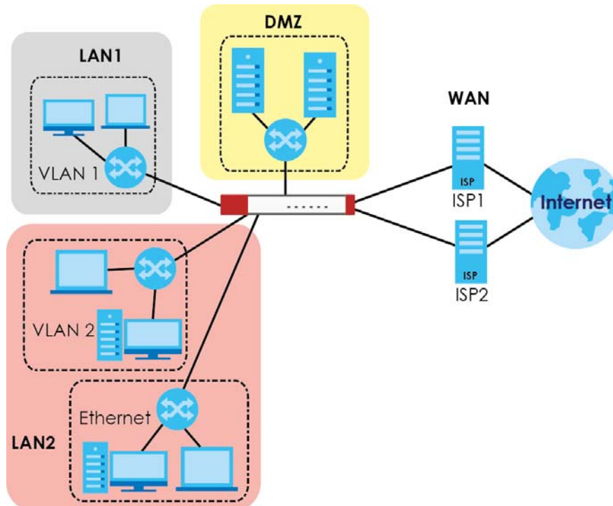
Figure 424 Example: Zones
