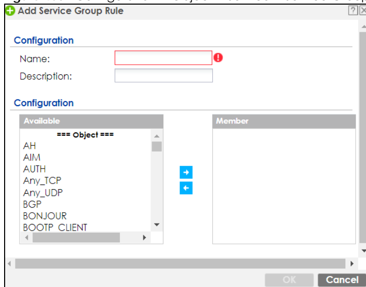
Figure 463 Configuration &gt; Object &gt; Service &gt; Service Group &gt; Edit
