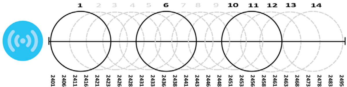
Figure 190 An Example Three-Channel Deployment
