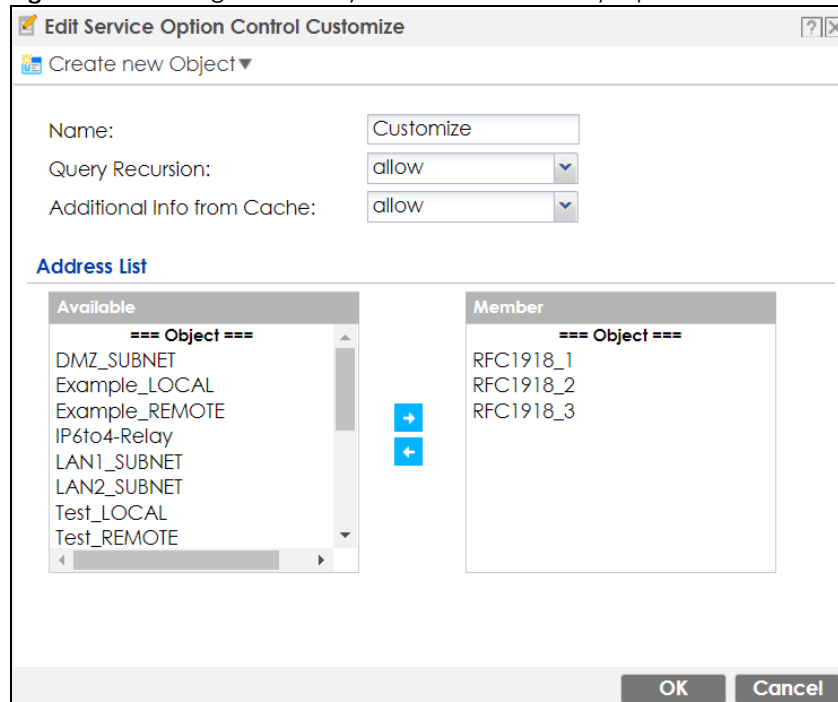
Figure 521 Configuration > System > DNS > Security Option Control Edit (Customize)
