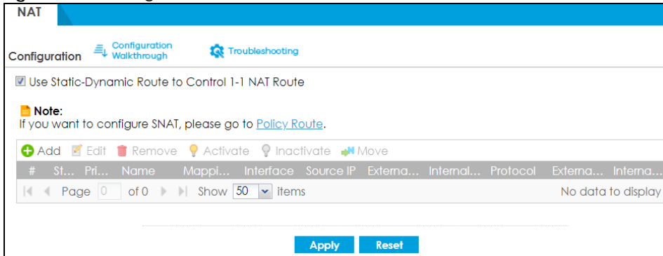
Figure 256 Configuration > Network > NAT
