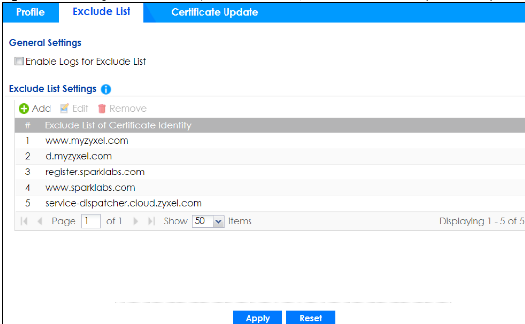
Figure 419 Configuration > Security Service > SSL Inspection > Exclude List (> Add/Edit)
