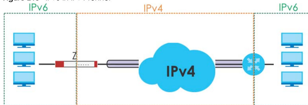
Figure 213 IPv6-in-IPv4 Tunnel
