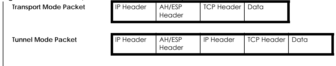
Figure 318 VPN: Transport and Tunnel Mode Encapsulation
