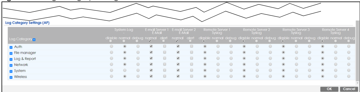
Figure 580 Log Category Settings AP
