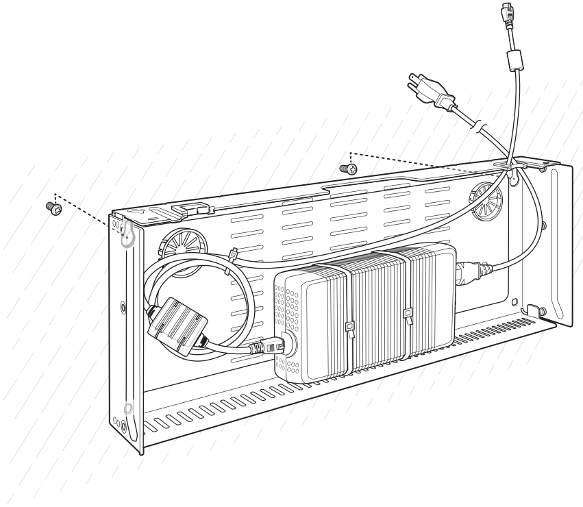
Figure 62 Vertical Installation
