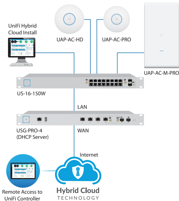
Sample Network Diagram
