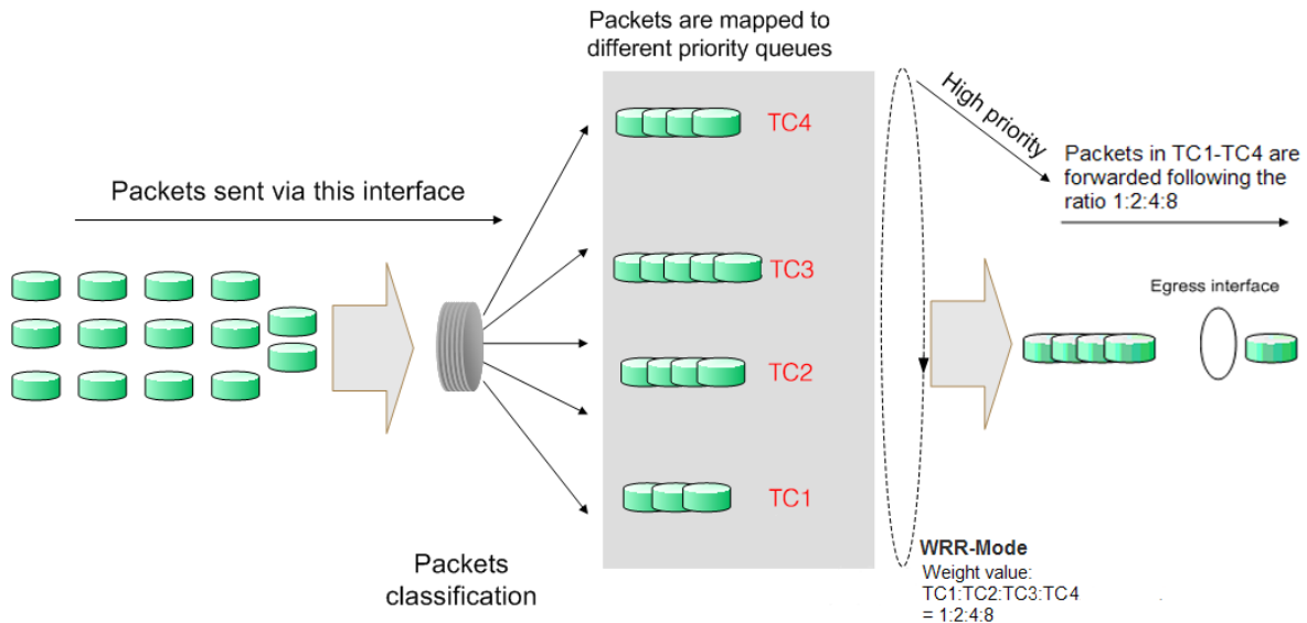
Figure 8-1 QoS function
