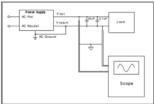
Figure 1. Ripple voltage test circuit
