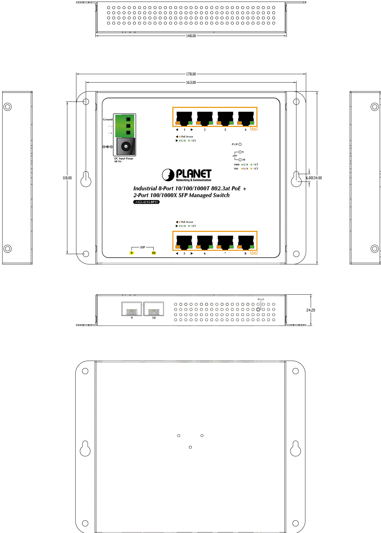
Dimensions (unit = mm)
