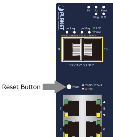
Figure 6-1: IGS-10020MT Reset Button
