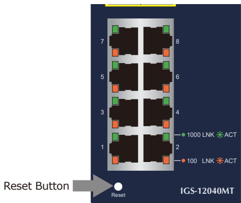
Figure 6-2: IGS-12040MT Reset Button
