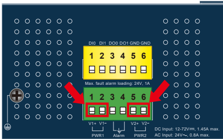
Figure 3-2: IGS-12040MT Upper Panel
