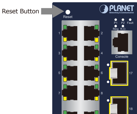
Figure 6-3: IGS-20040MT Reset Button
