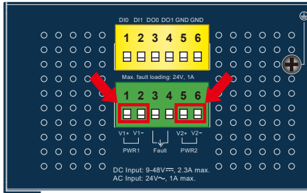
Figure 3-3: IGS-20040MT Upper Panel
