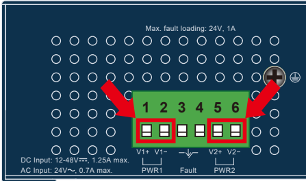
Figure 3-1: IGS-10020MT Upper Panel
