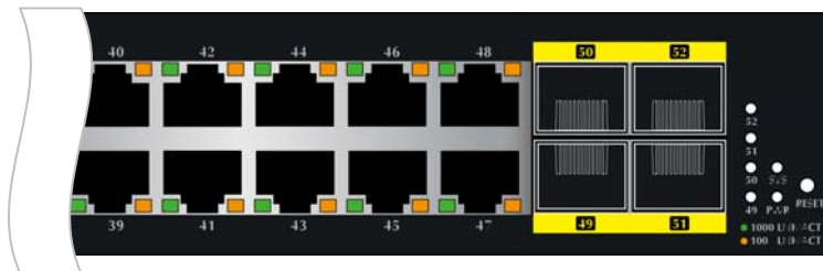
Figure 2-1-2d GS-4210-48T4S LED Panel
