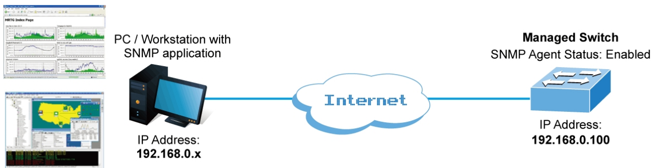
Figure 3-1-5 SNMP Management
