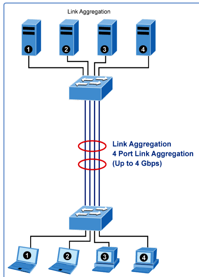
Figure 4-4-1 Link Aggregation
