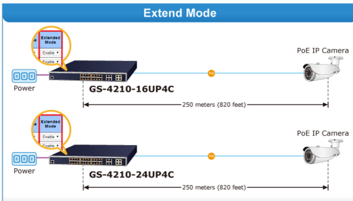
10BASE-T UTP with PoE
