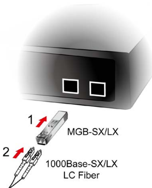
Figure 2-1-7 Plug in the SFP transceiver
