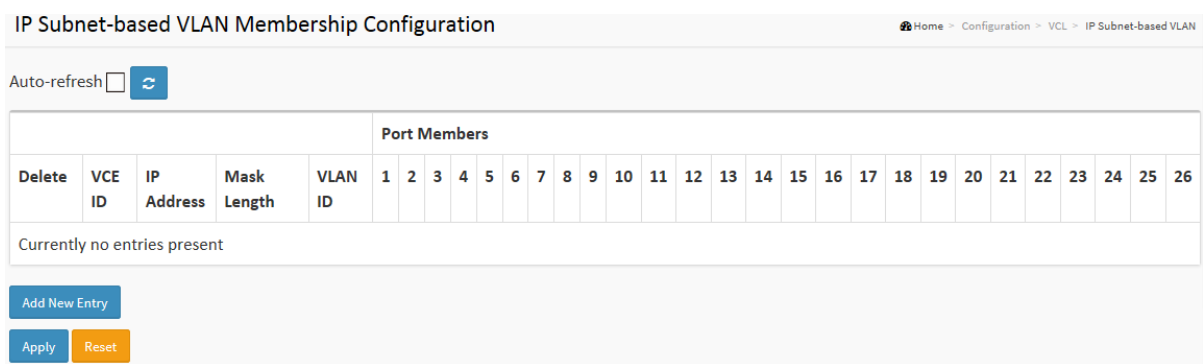
Figure 2-17.3: IP Subnet-based VLAN Membership Configuration
