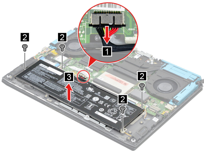
Figure 6. Remove the battery pack (on selected models)
