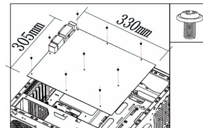
Motherboard mounting on the tray
