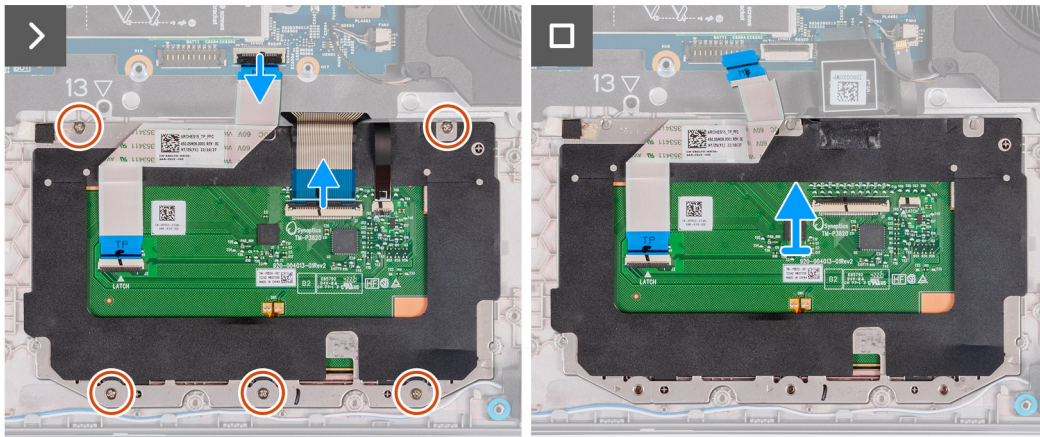
5x M2x2.5
