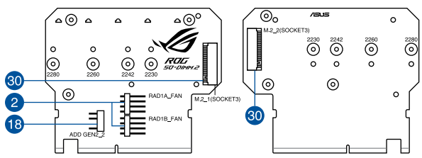
SO-DIMM.2 card
