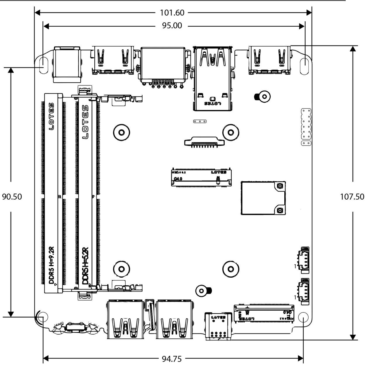
Figure 17. Board Dimensions
